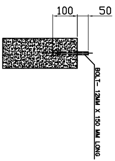
ELEVATION OF BOLT
